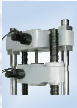
SF309 油壓拉力夾具 Hydraulic Grips
